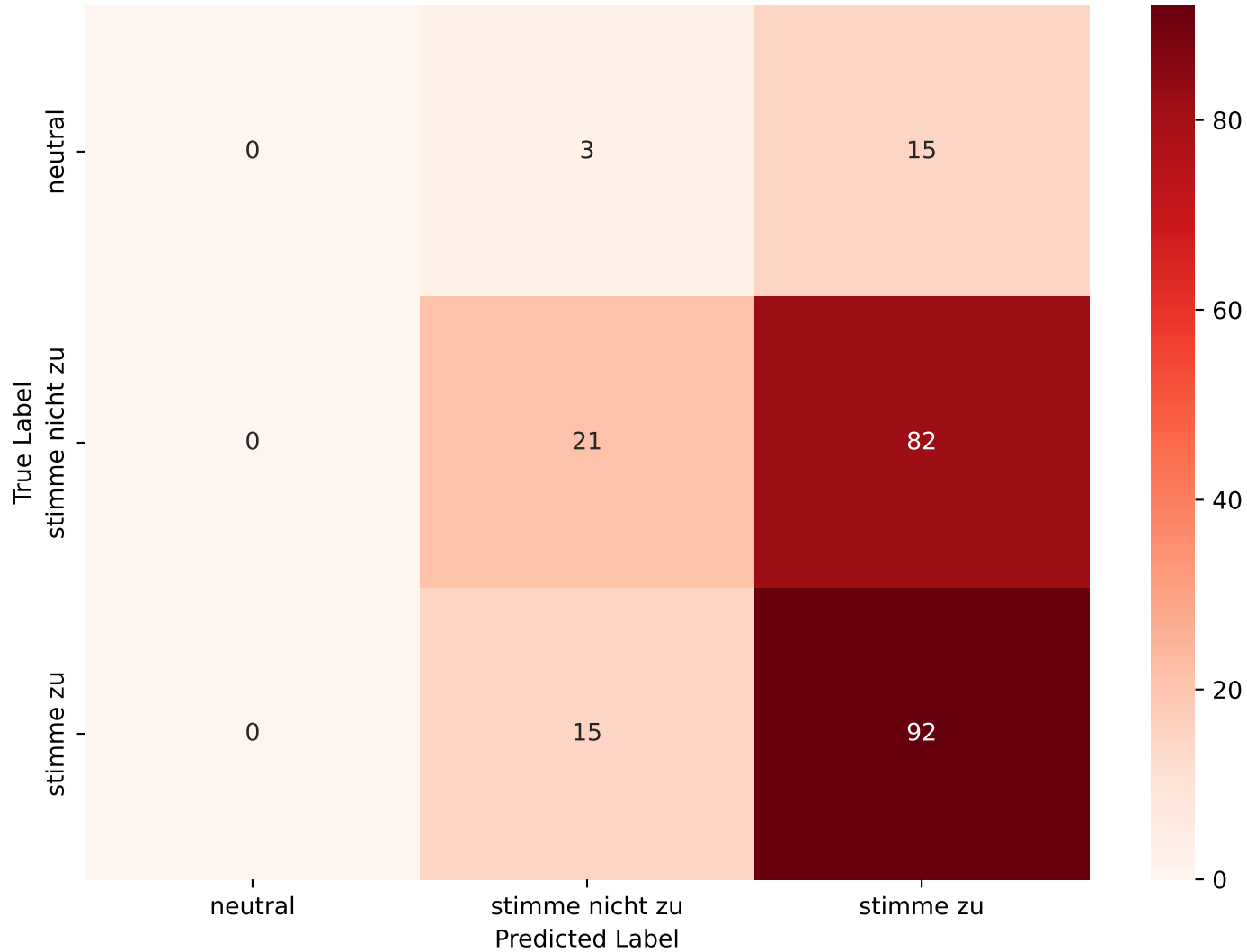
Confusion Matrix - Llama 3, temp: 0.3
